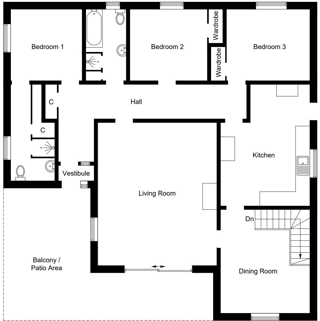
Ground Floor
