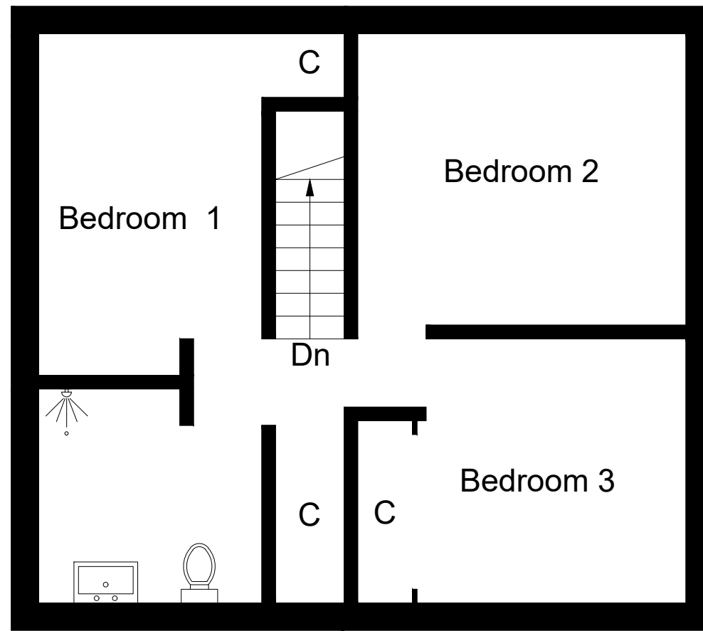
First Floor
